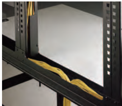
Organizer Frames offer both horizontal and vertical integrated cable management.
