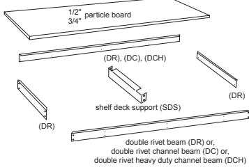
Bottom Shelf
