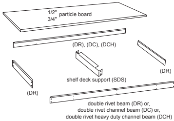
Top Shelf
