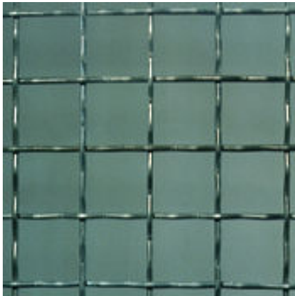
2" square opening 6 gauge (.192)
