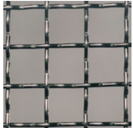
1-1/2" square opening 8 gauge (.162)
